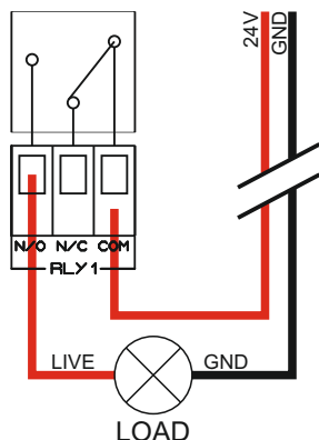
Relay connection when relay is not energised
